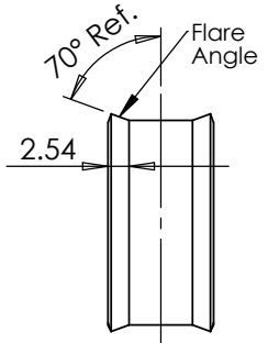
Section B-B Vinyl Coating Removed
